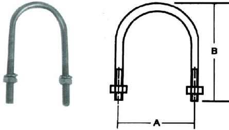
Type UB U型螺栓 U-Bolts
